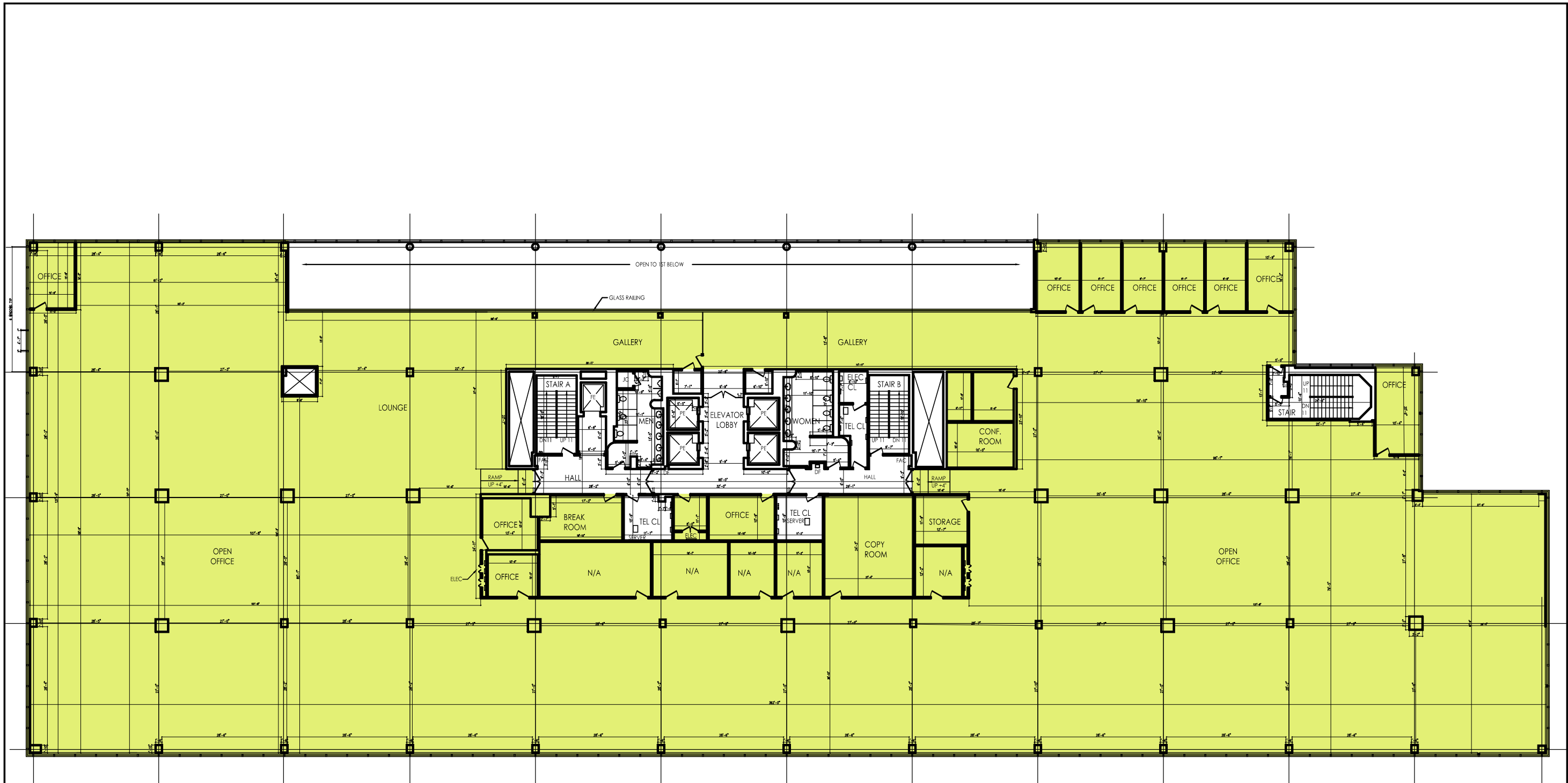
5 900 STEWART AVE. 5TH FLOOR PLAN TENANT SPACE: 35,502 SF 3/32" = 1'-0" CORE: 3,741 SF GROSS: 39,243 SF
